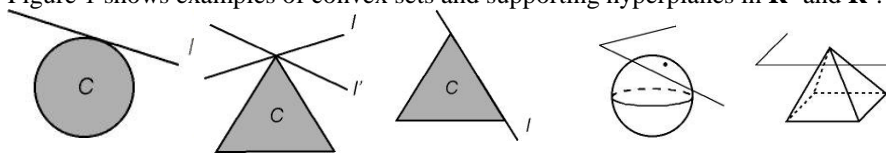
Figure 1: Examples of closed convex sets and hyperplanes
