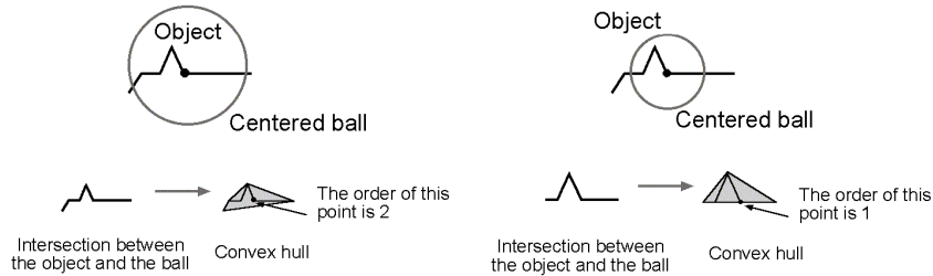
Figure 4: Determination of the order of a broken line's point with different ball radius.
