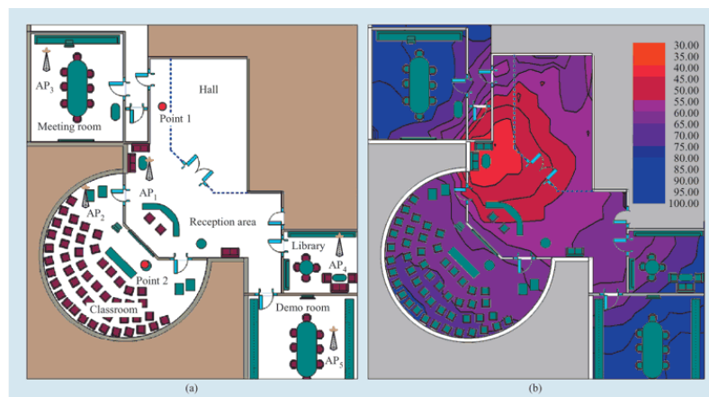
Figure 6: Layout testarea (a) and Contours (b) indicating the signal strength of Access Points
