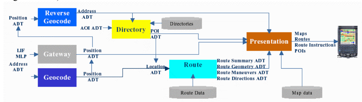
Figure 1: Request/response of GeoMobility Server as the position is provided by the communication network
