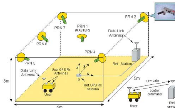
Figure 3: Centimeter-Accuracy Indoor Navigation Using GPS-Like Pseudolites
