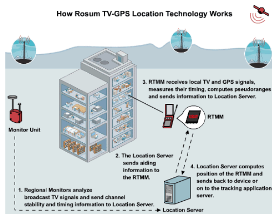
Figure 4: Rosum TV-GPS Location Technology
